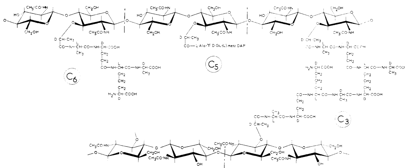
FIGURE 1: Structure of a fragment of the E. coli B peptidoglycan representing the disaccharide tripeptide: C 5 , the disaccharide tetrapeptide: C 6 and the dimer of C 6 , bis(disaccharide tetrapeptide): C 3 .
