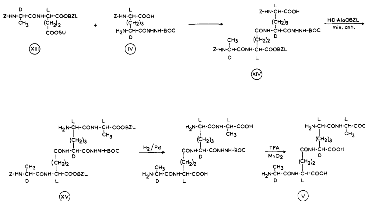
FIGURE 4: Synthesis of the tetrapeptide: D-Ala- \gamma -L-Glu-(D) meso -DAP(L)-L-Ala(V).
