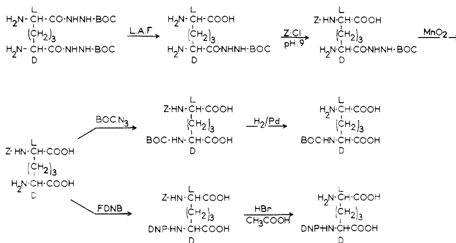
FIGURE 5: Stereospecific synthesis of Z-(L) meso -DAP(D)-NHNH- t -butyloxycarbonyl and of DNP-(D) meso -DAP.
