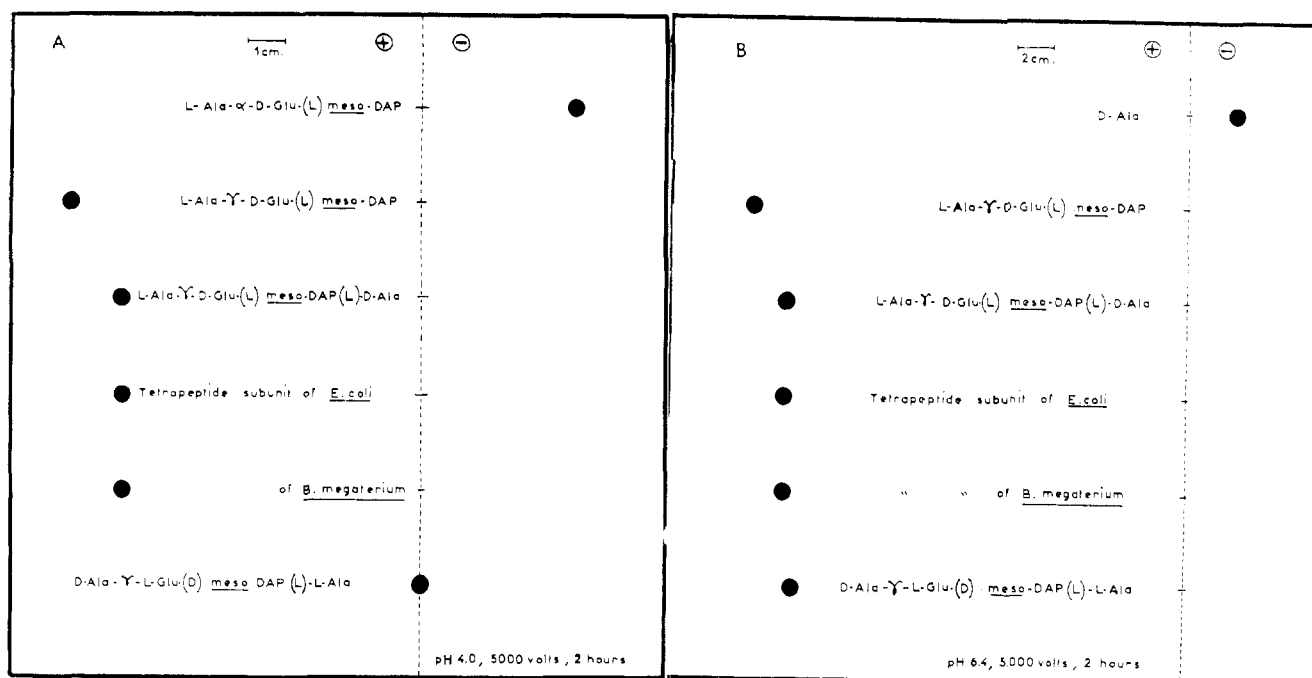
FIGURE 6: High-voltage paper electropherograms at pH 4.0 (A) and at pH 6.4 (B) of the isomeric synthetic tri- and tetrapeptides and the corresponding natural tetrapeptide subunits of the cell wall peptidoglycans of E. coli B and B. megaterium KM.
