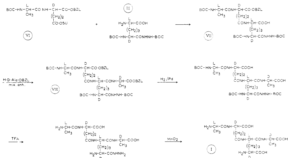
FIGURE 2: Synthesis of the tetrapeptide: L-Ala-γ-D-Glu-(L)meso-DAP(L)-D-Ala (I).
