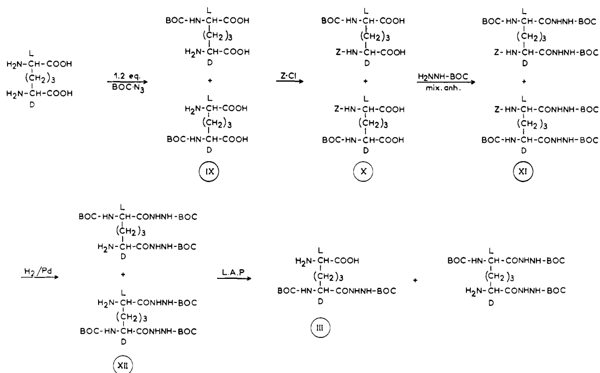
FIGURE 3: New method of preparation of stereospecific N -monoacylated derivatives of meso -DAP: Synthesis of t -butyloxycarbonyl- ( D ) meso -DAP( D )-NHNH- t -butyloxycarbonyl (III).
